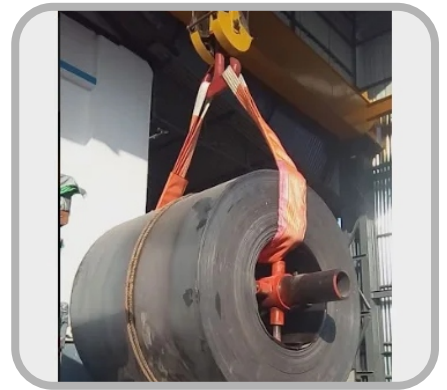
Coil Lifting Sling
